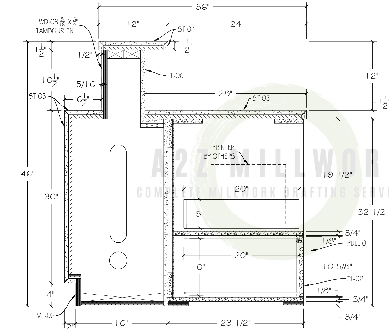
A VERT. SECT. 01.12 SCALE: 1 1/2" = 1'-0" N/A
