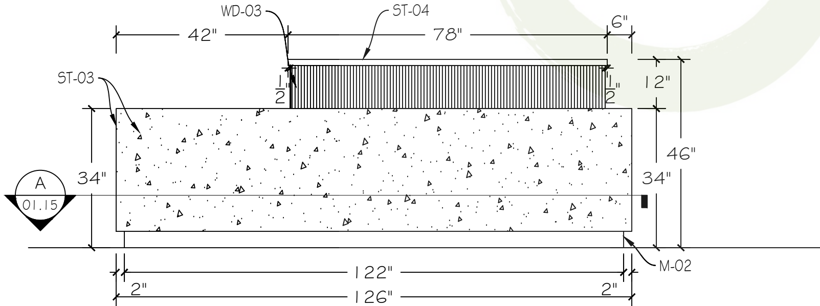
2 ELEVATION @ FRONT DESK 122 01.02 SCALE: 1/2"=1'-0" 2/15.00
