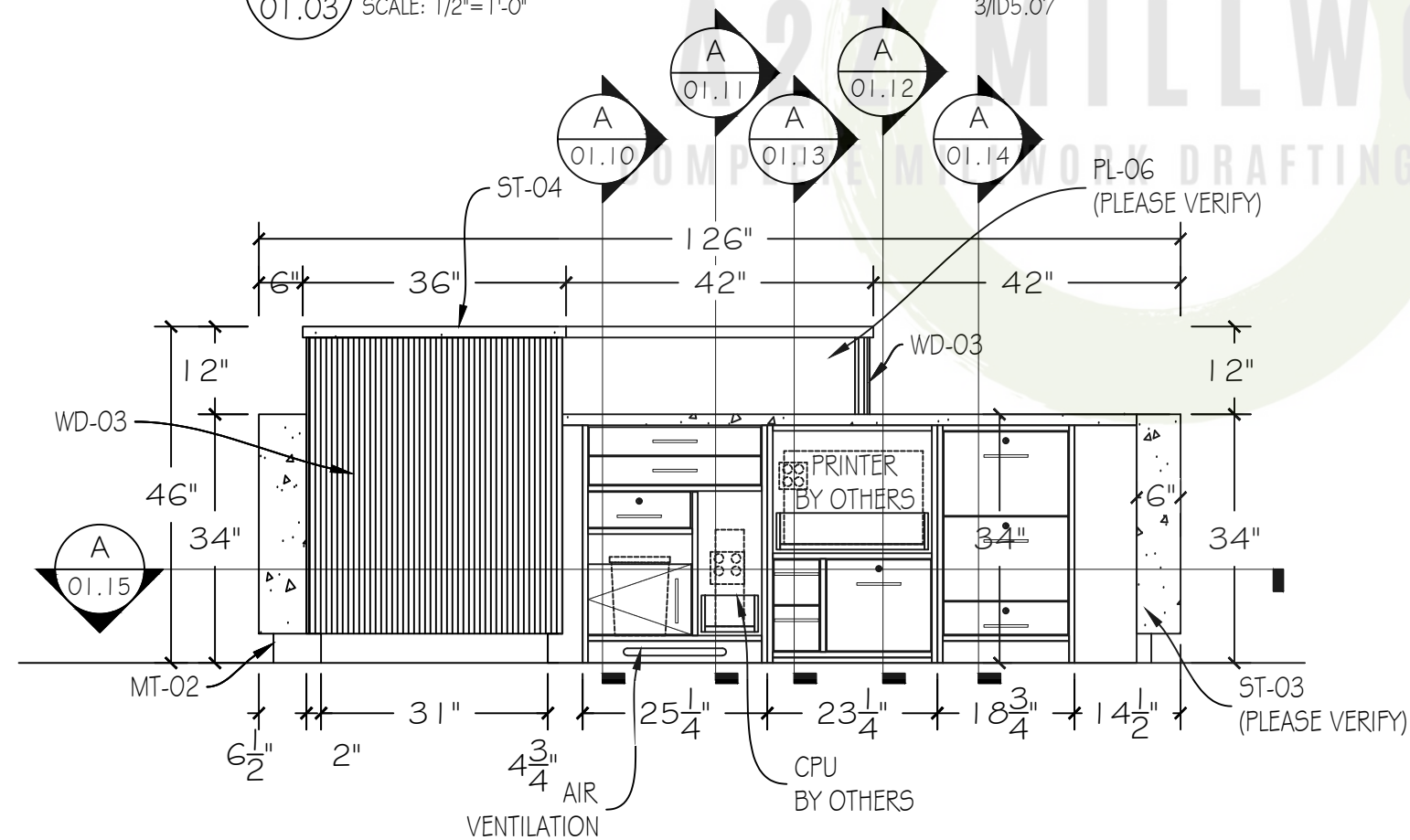
2 ELEVATION @ FRONT DESK 122 01.03 SCALE: 1/2"=1'-0" 2/10/2023
