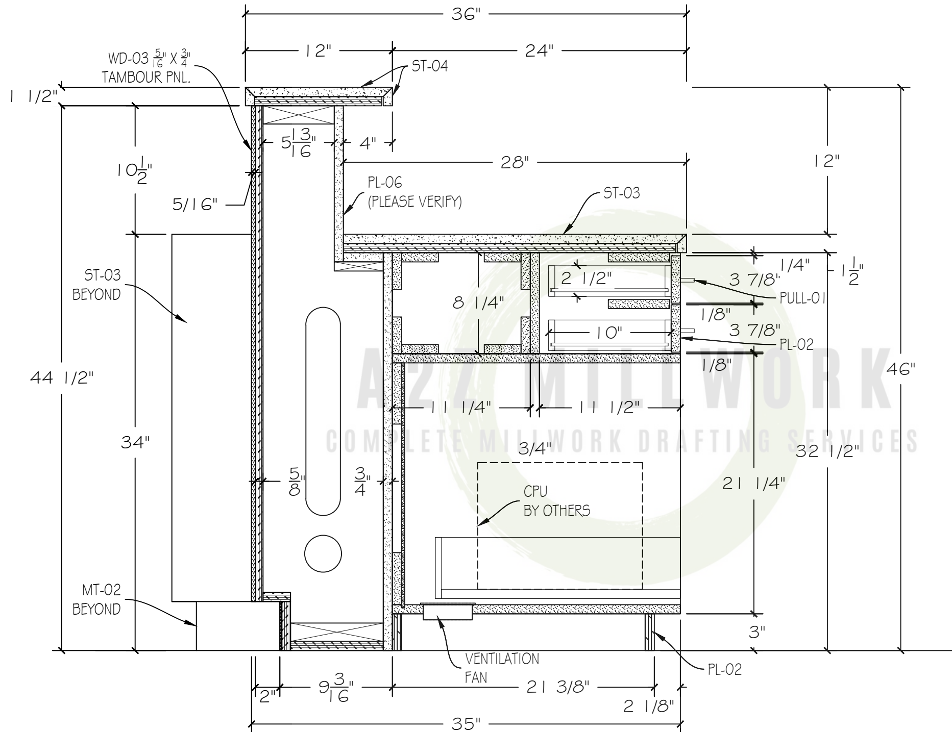
A VERT. SECT. 01.06 SCALE: 1 1/2" = 1'-0" N/A
