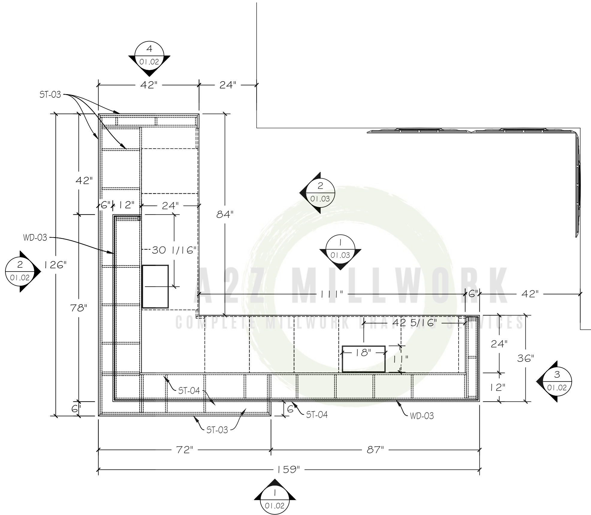
1 PLAN @ FRONT DESK 122 01.01 SCALE: 1/2"=1'-0" 1/12.00
