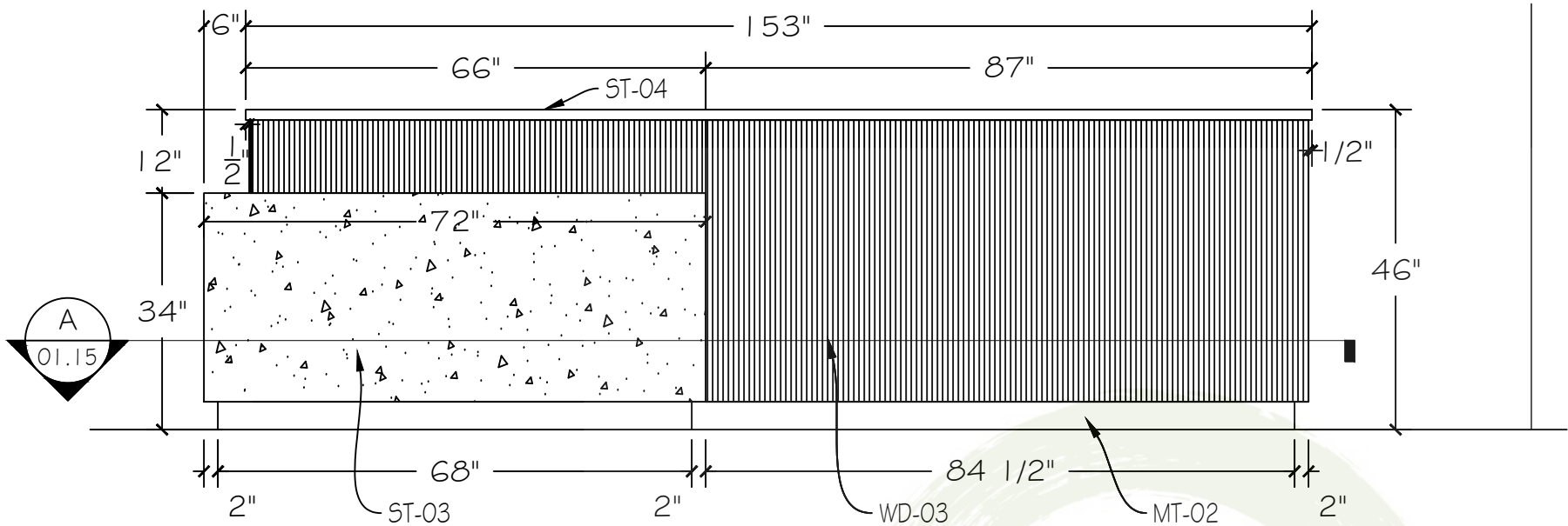
1 ELEVATION @ FRONT DESK 122 01.02 SCALE: 1/2"=1'-0" 1/15.00
