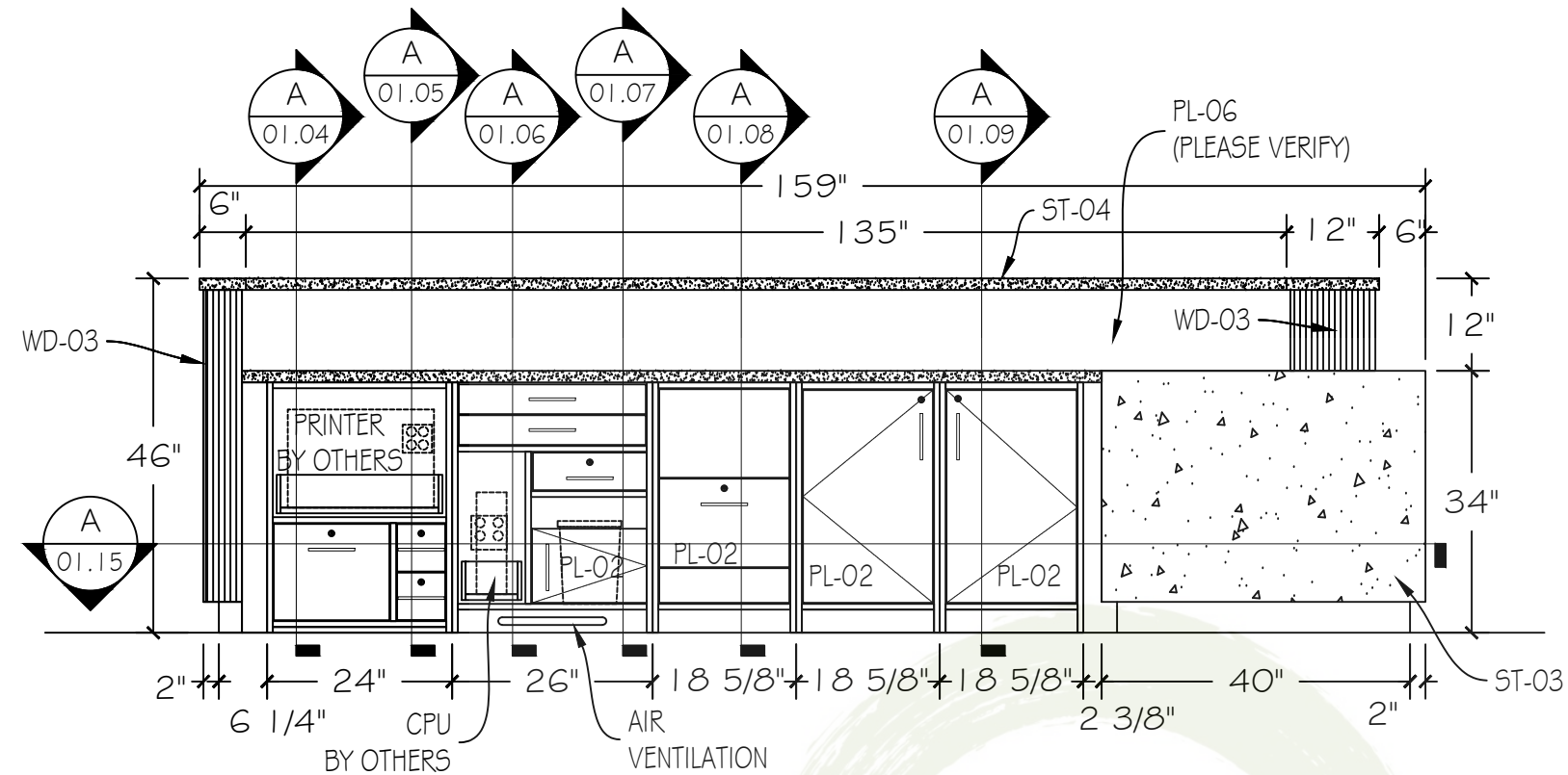
1 ELEVATION @ FRONT DESK 122 01.03 SCALE: 1/2"=1'-0" 3/10/2023
