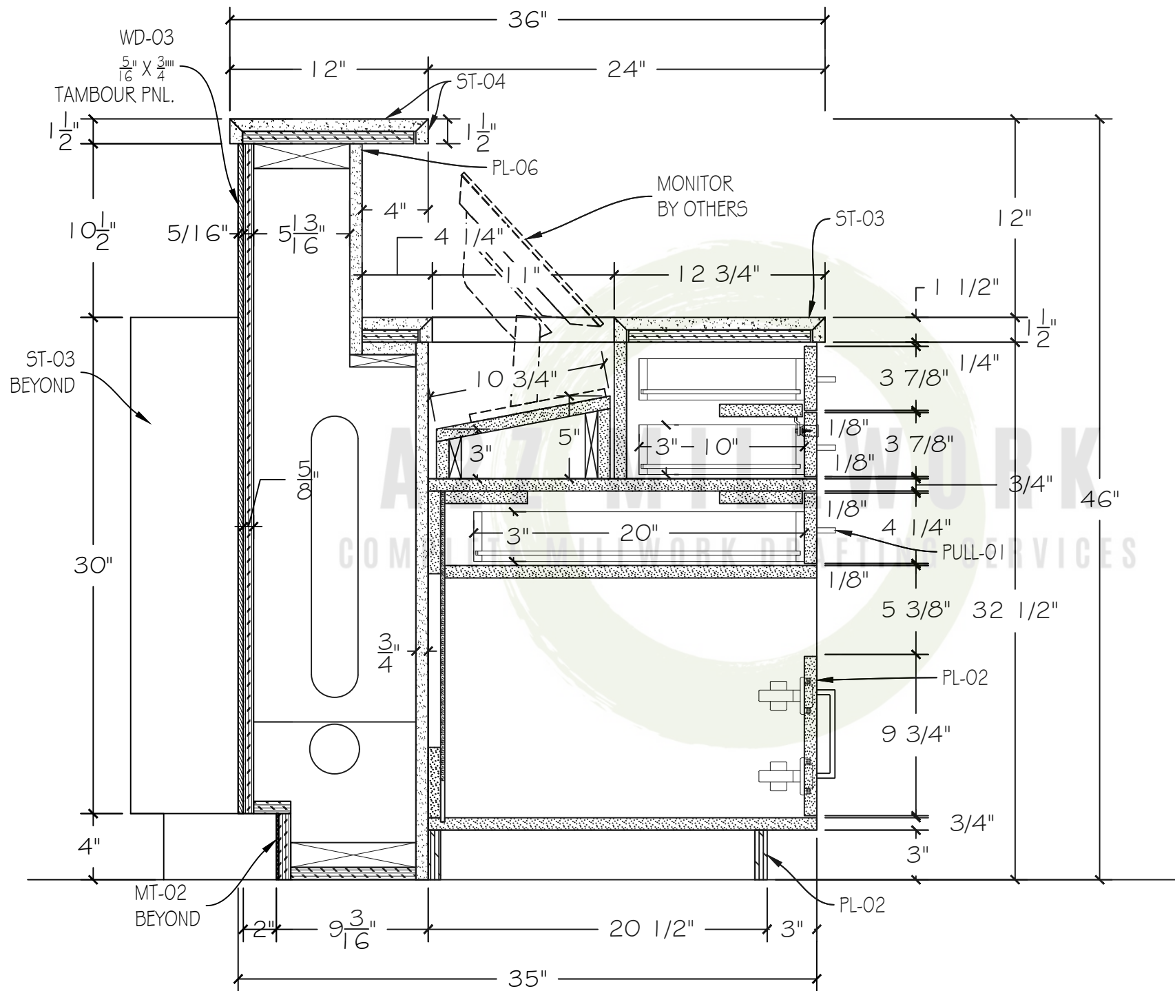
A VERT. SECT. 01.07 SCALE: 1 1/2" = 1'-0" N/A
