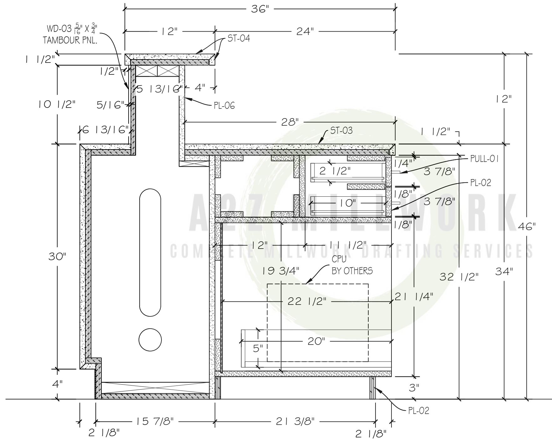
A VERT. SECT. 01.13 SCALE: 1 1/2" = 1'-0" N/A
