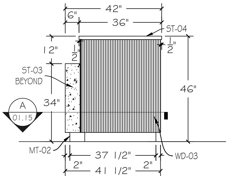
3 ELEVATION @ FRONT DESK 122 01.02 SCALE: 1/2"=1'-0" 2/15.07
