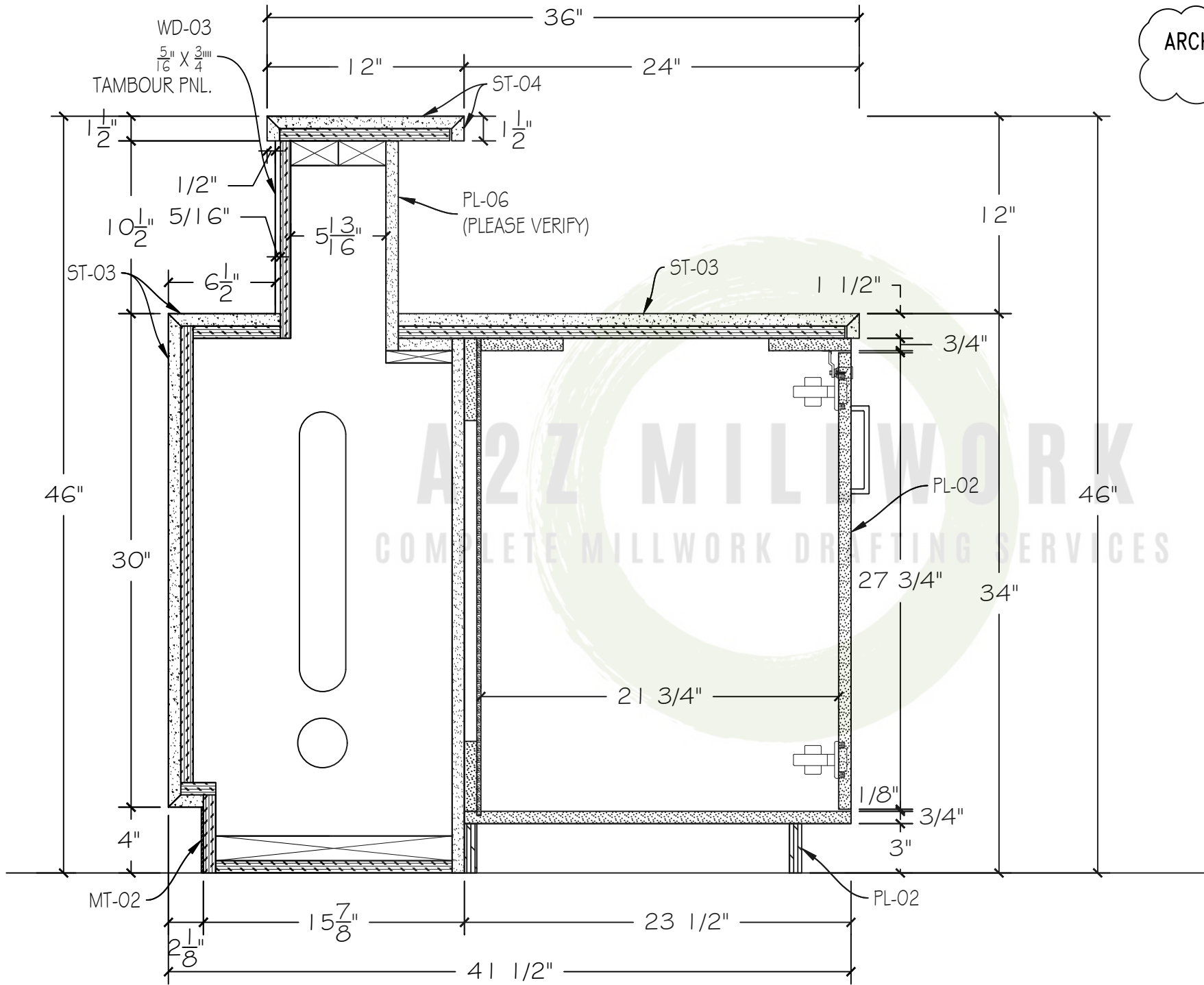
A VERT. SECT. 01.09 SCALE: 1 1/2" = 1'-0" N/A
