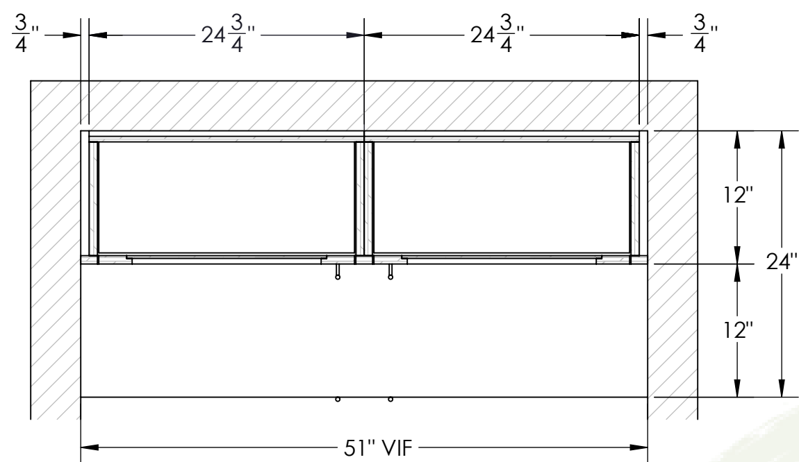
M 4.1 PLAN SECTION - PANTRY SCALE - 1:12
