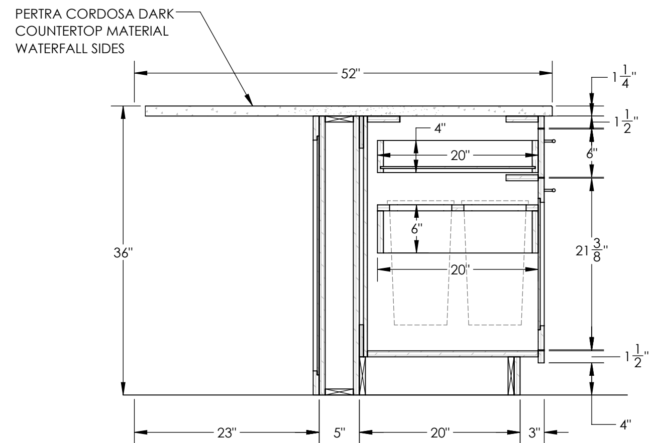
E 2.1 SECTION - KITCHEN ISLAND SCALE 1:12
