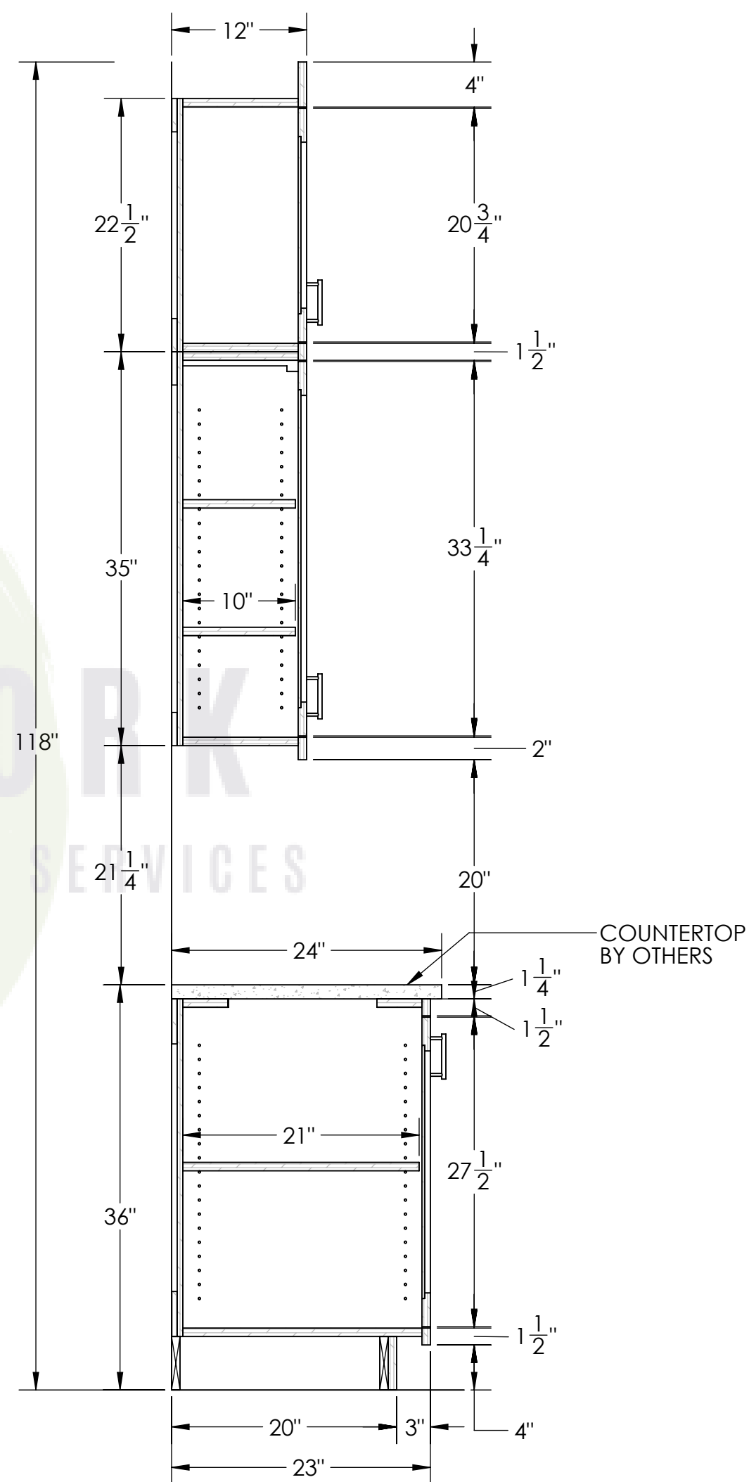
O 4.1 SECTION - PANTRY SCALE - 1:12
