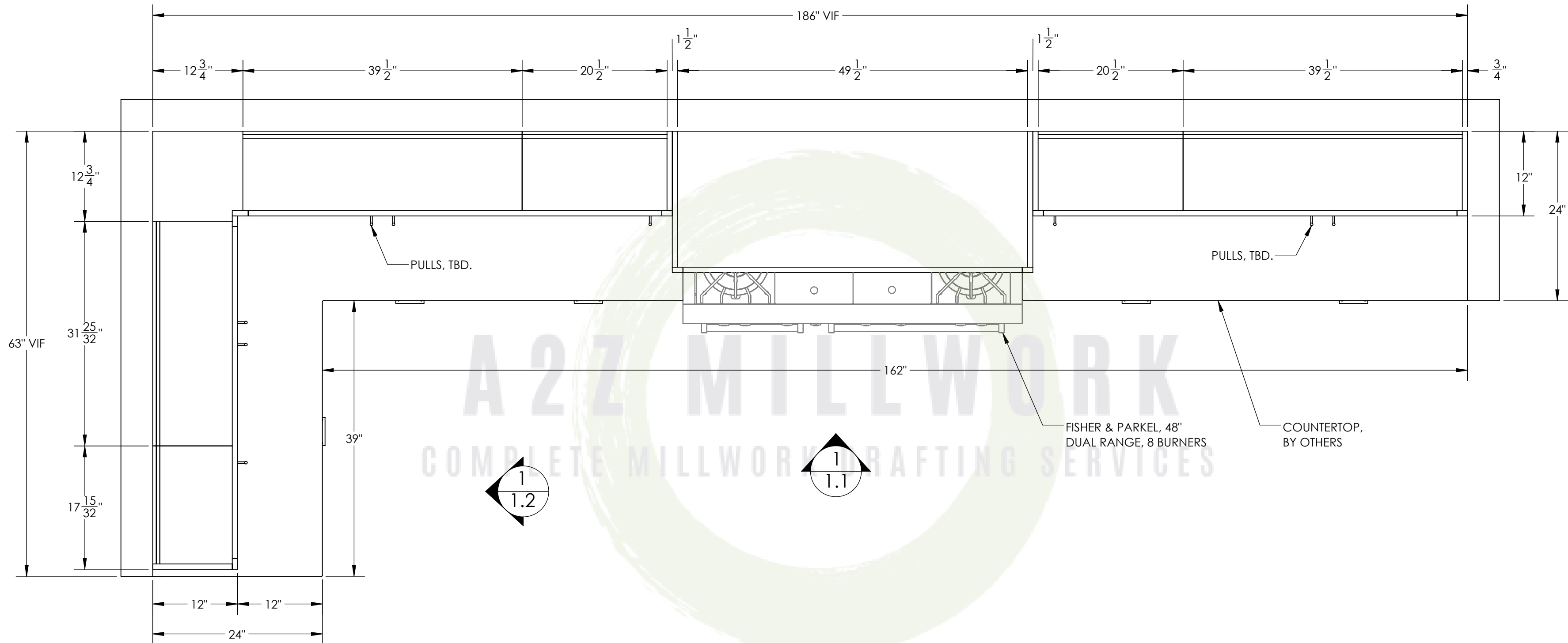
1 PLAN - KITCHEN 1.0 SCALE - 1:12
