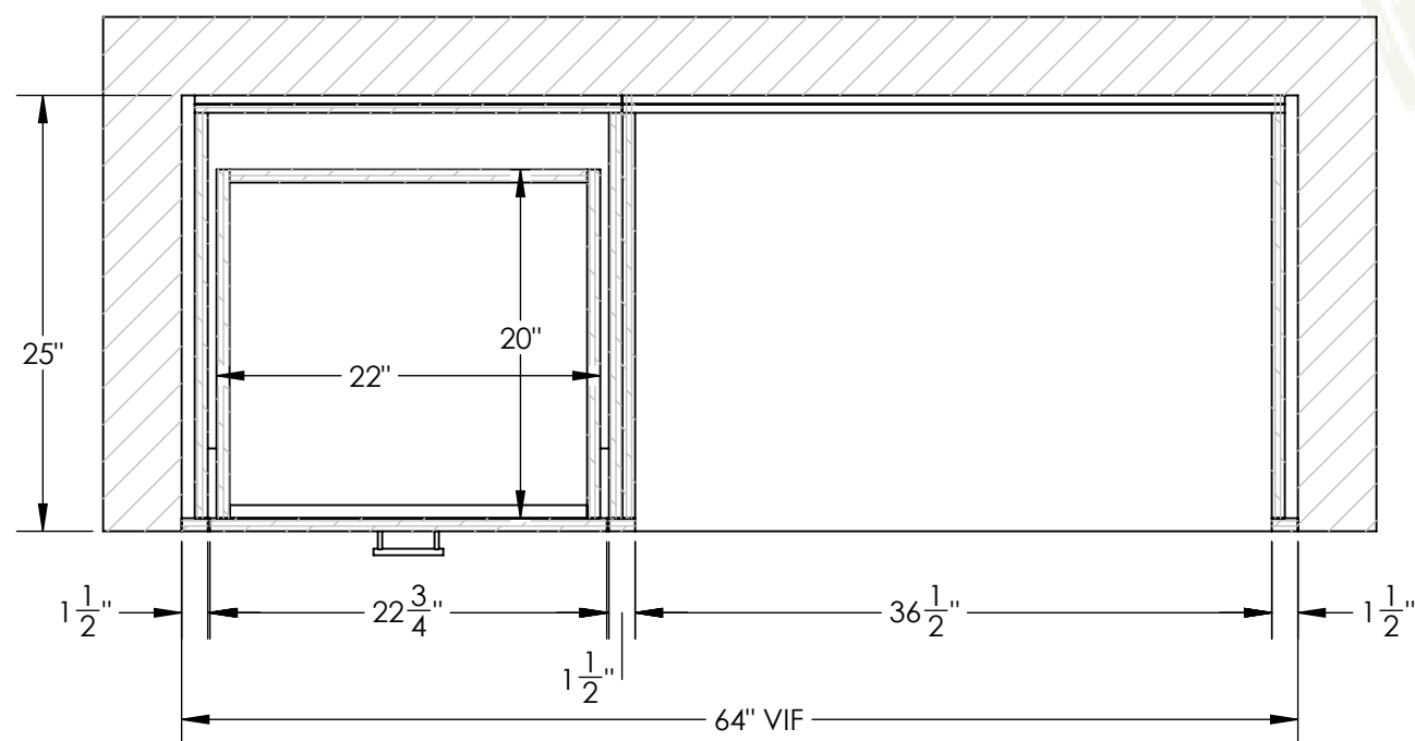
K SECTION - BEVERAGE & REF. AREA 3.1 SCALE - 1:12
