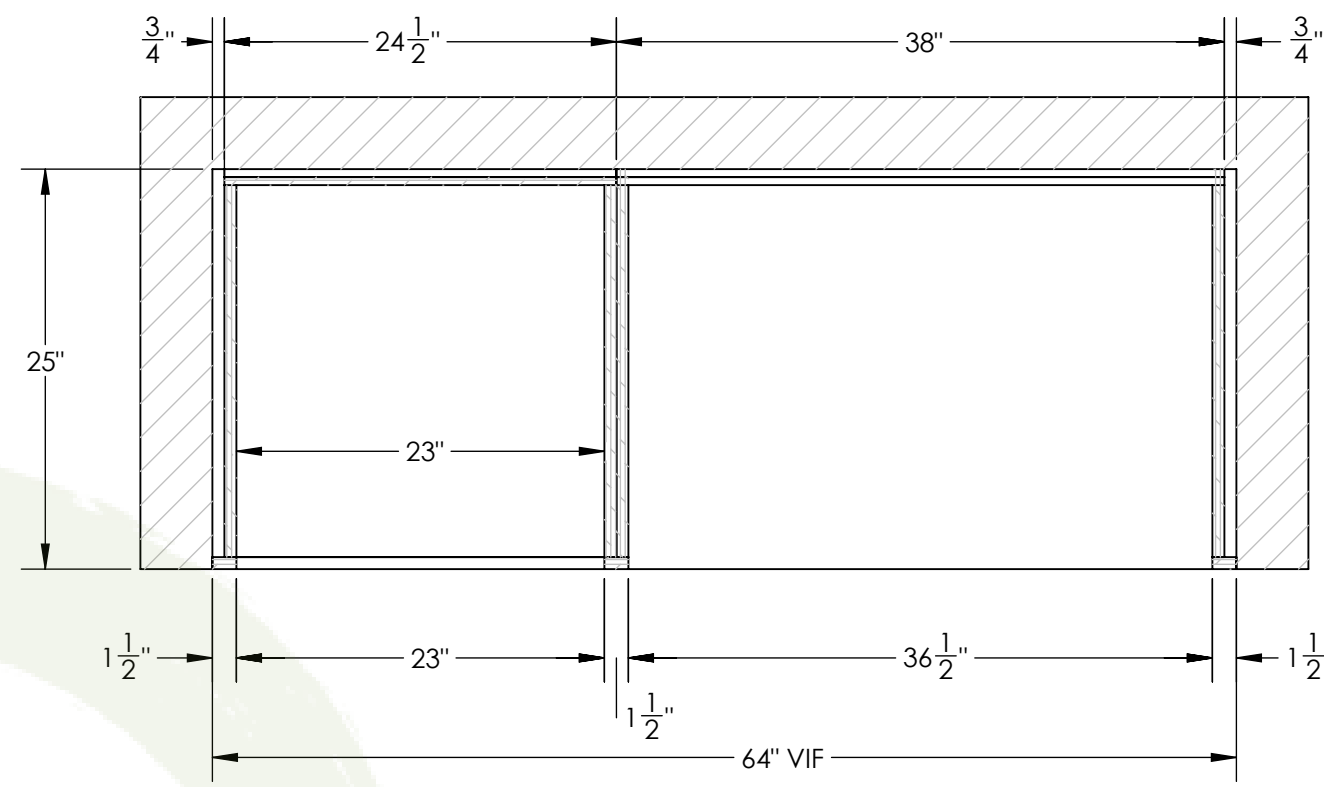
J SECTION - BEVERAGE & REF. AREA 3.1 SCALE - 1:12
