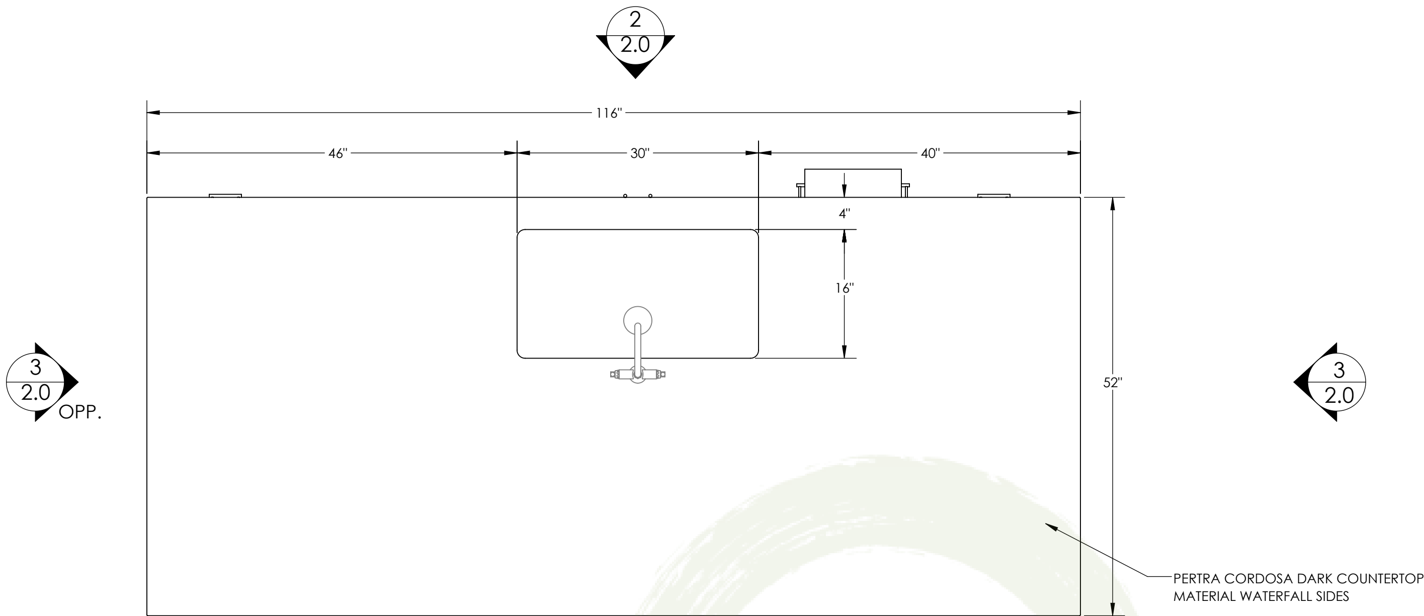
1 2.0 PLAN - KITCHEN ISLAND SCALE - 1:12
