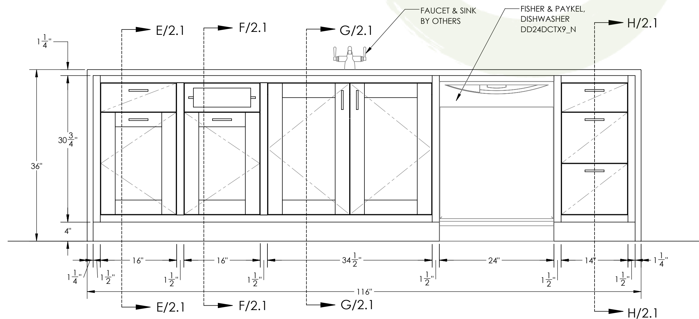
2 2.0 ELEVATION - KITCHEN ISLAND SCALE - 1:12
