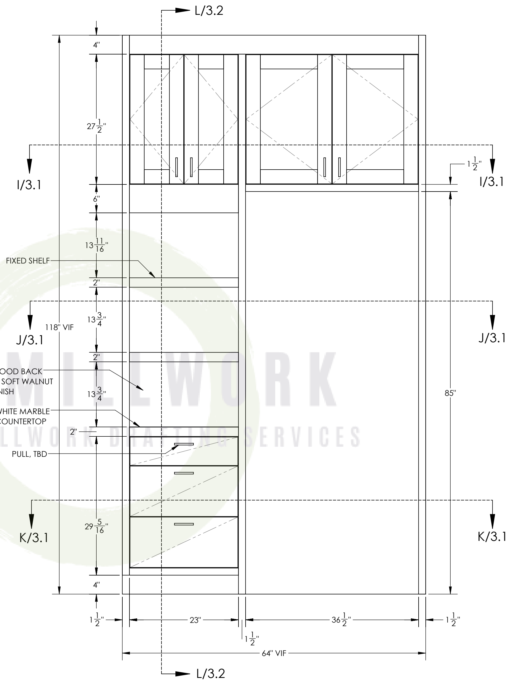
1 3.0 ELEVATION - BEVERAGE & REF. AREA SCALE - 1:12
