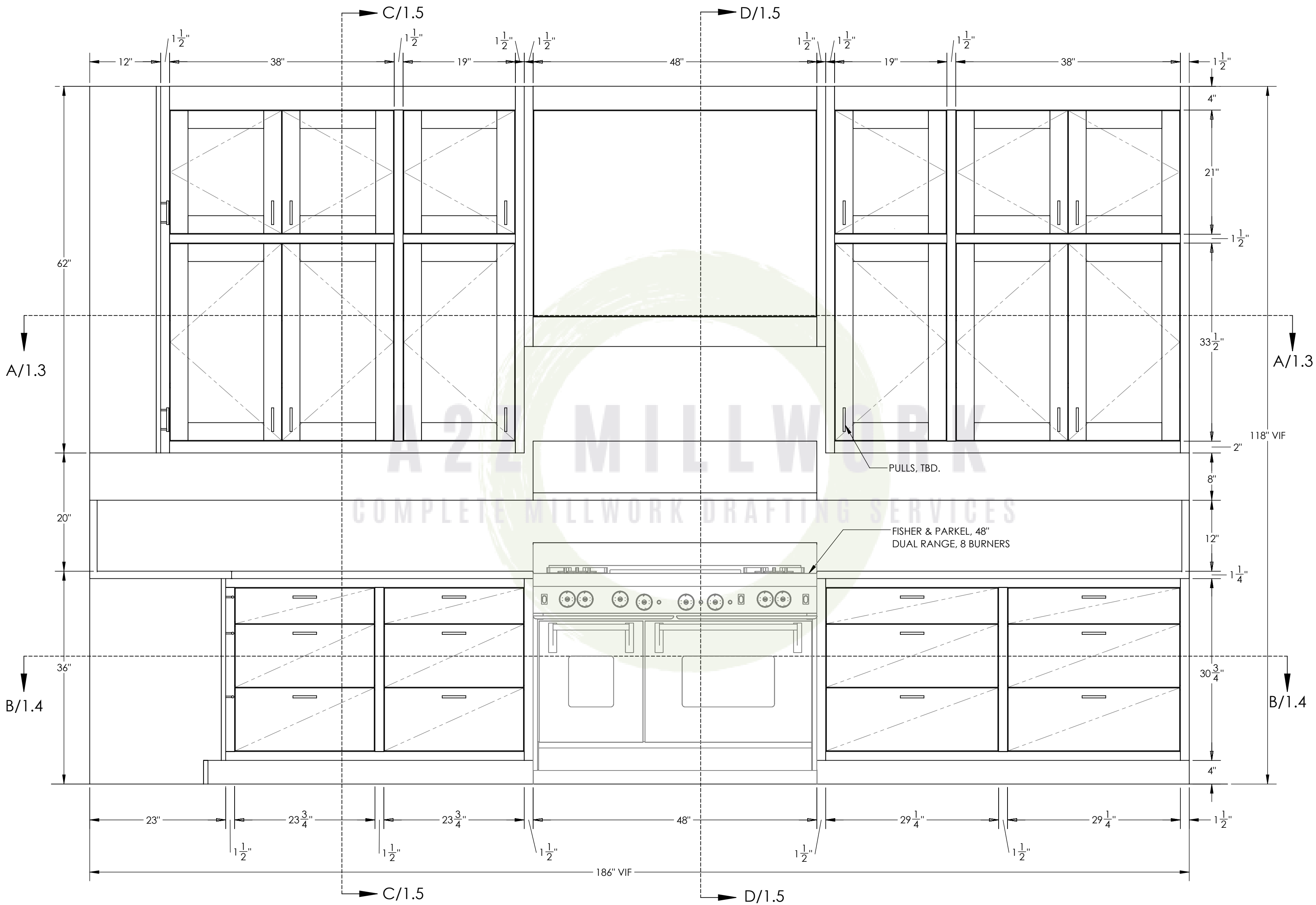
1 1.1 ELEVATION - KITCHEN SCALE - 1:12
