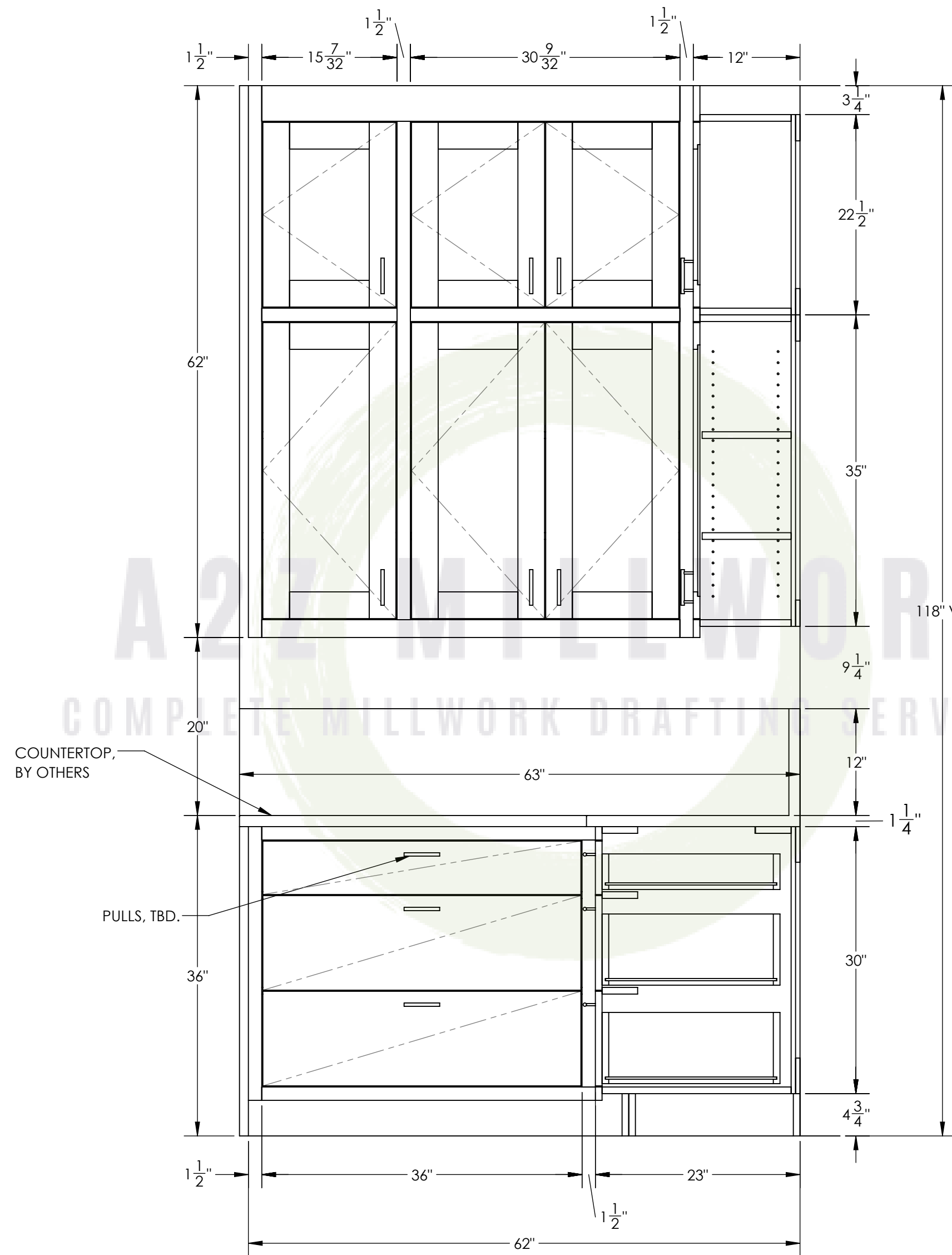
1 ELEVATION - KITCHEN 1.2 SCALE - 1:12
