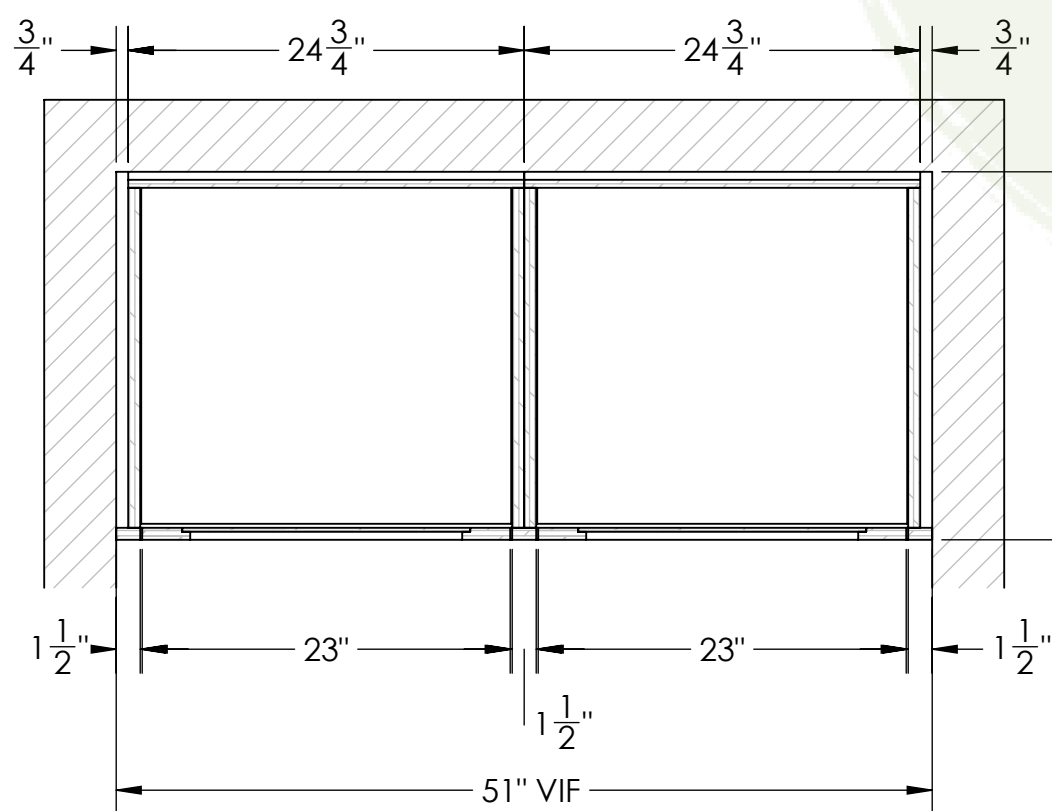
N 4.1 PLAN SECTION - PANTRY SCALE - 1:12
