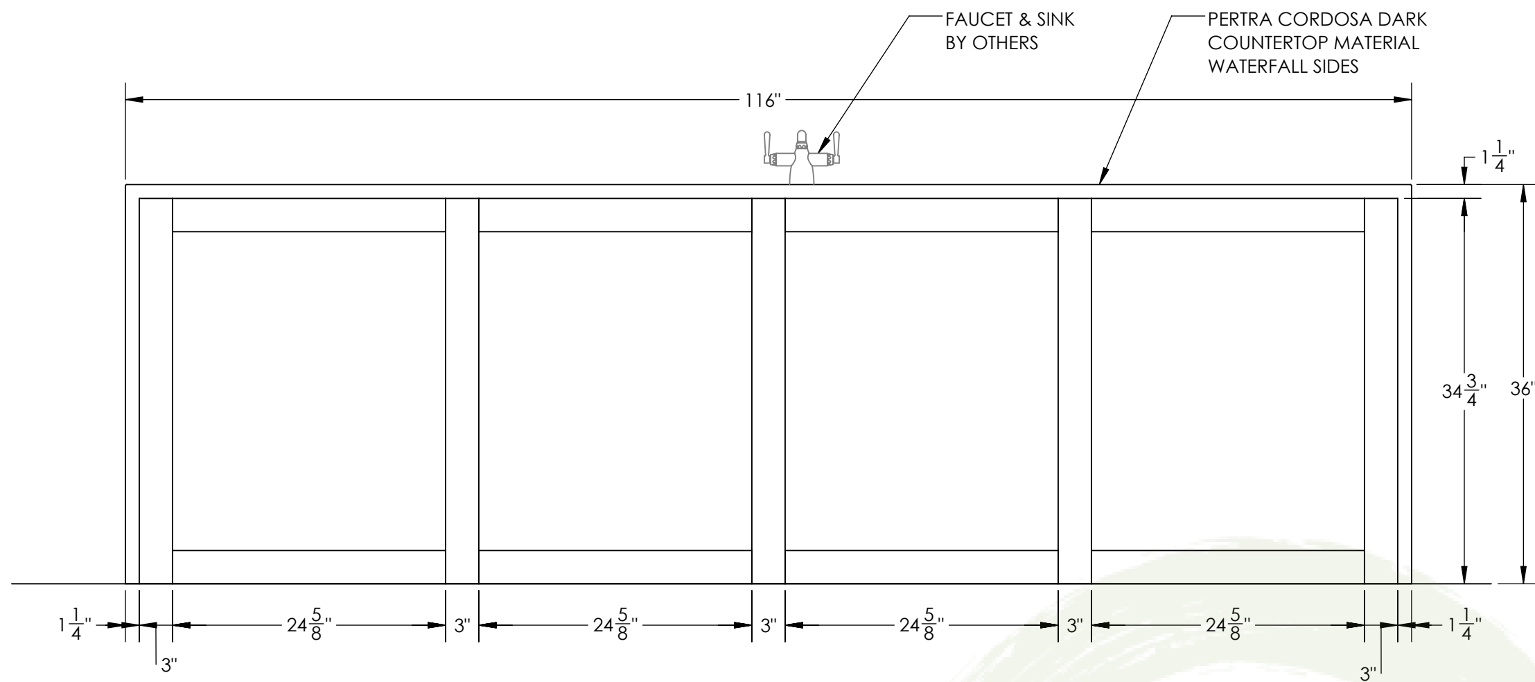
1 2.1 ELEVATION - KITCHEN ISLAND SCALE 1:12
