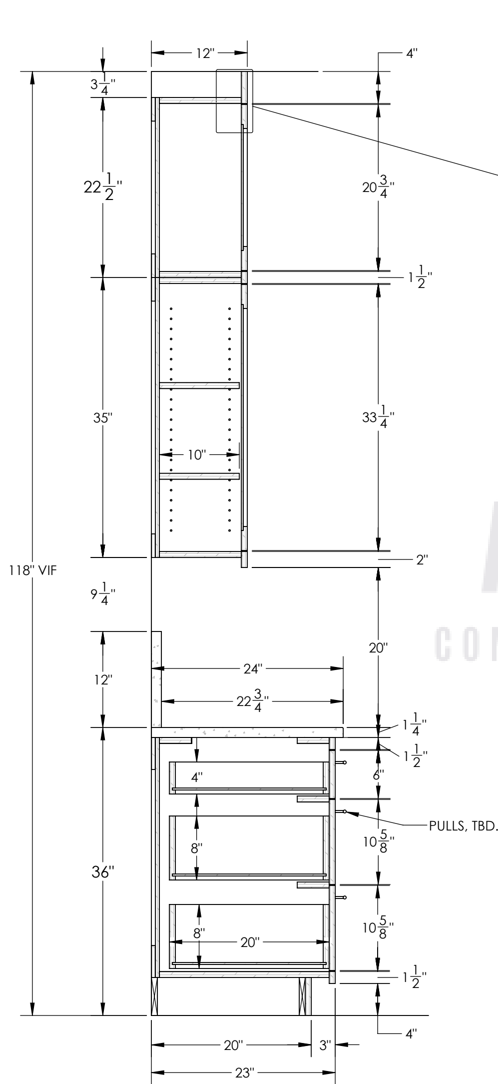
C SECTION - KITCHEN 1.5 SCALE - 1:12
