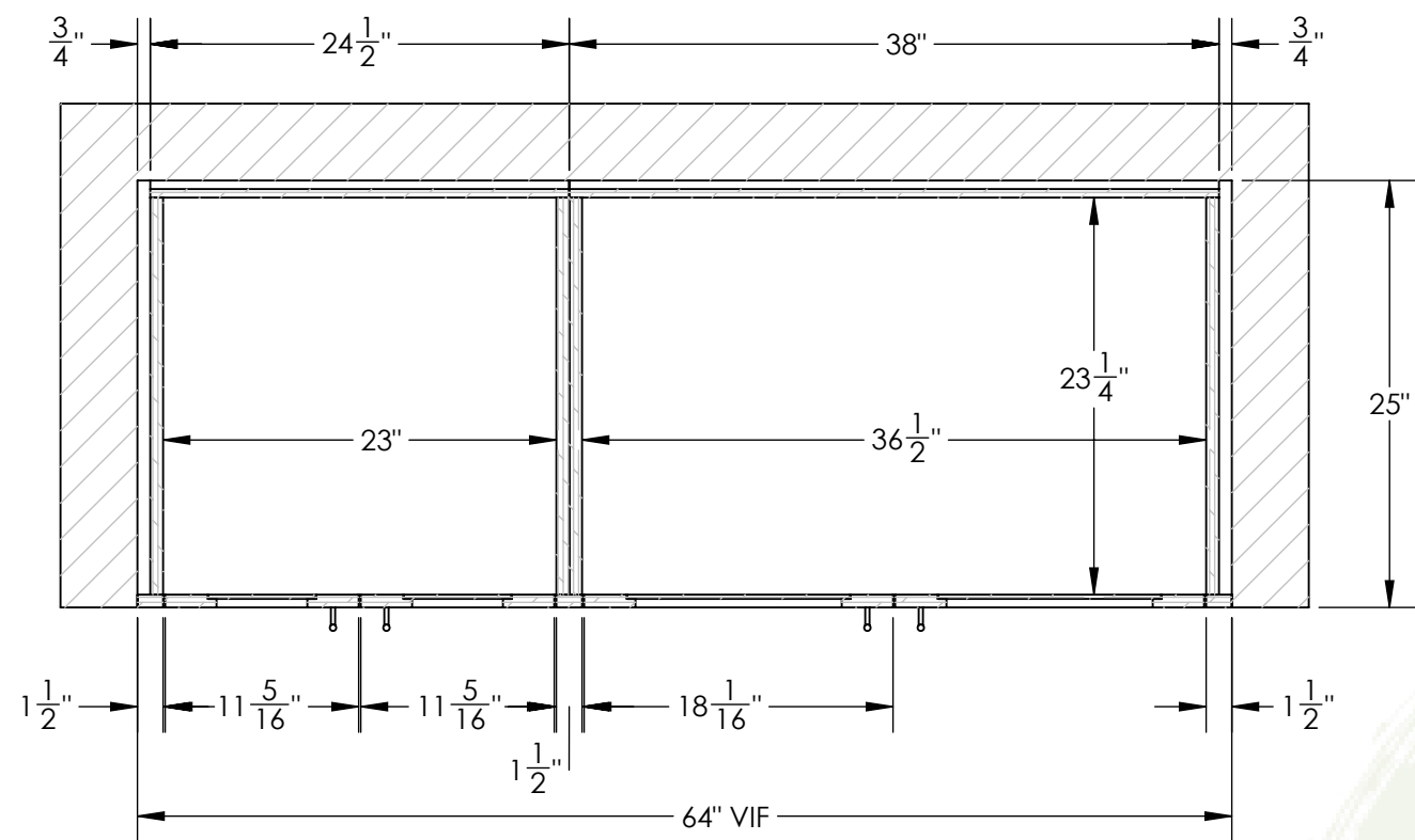
I SECTION - BEVERAGE & REF. AREA 3.1 SCALE - 1:12
